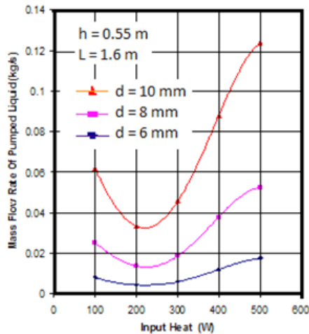
Figure (9) The variation of mass flow rate of pumped liquid for h = 0.55 m and L = 1.6 m; the present study.
